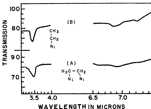
FIG. 22. A, spectrum of ethylene chemisorbed on hydrogen-covered nickel; B, after treatment with hydrogen. From Eischens and Pliskin (41); reproduced by permission of Academic Press, Inc.
