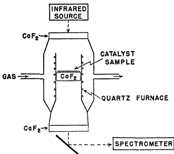
FIG. 19. Cell for infrared study of chemisorbed gases. Adapted from Eischens (39); reproduced by permission of the American Chemical Society.
