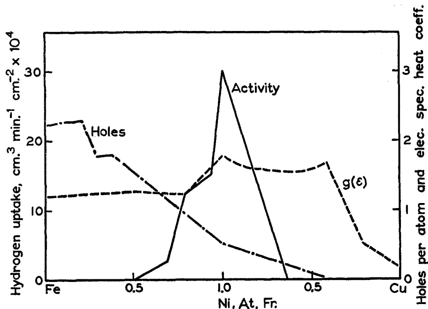
FIG. 8. Hydrogenation of styrene over nickel alloyed with iron and with copper. Adapted from Dowden and Reynolds (34); reproduced by permission of the Faraday Society and the authors.
