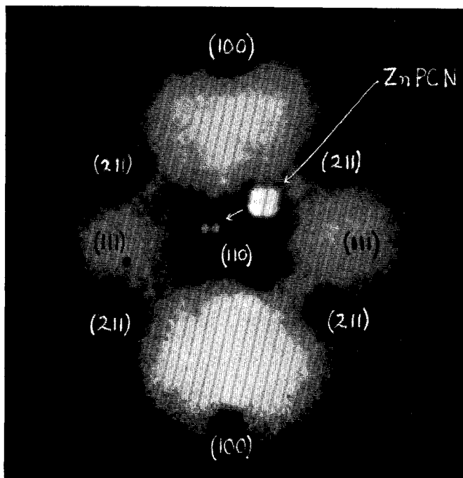
FIG. 18. Field emission microscope pattern produced by a tungsten tip. Reproduced by permission of R. Gomer.
